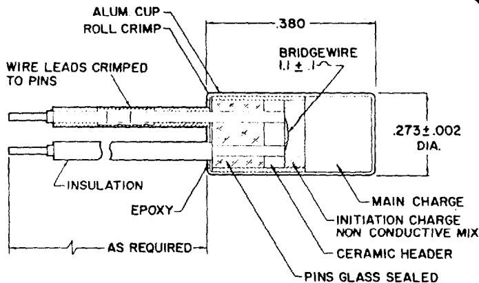
Fig 1 Cross-section through a Squib (1 amp/1 watt) (from Ref 3)
